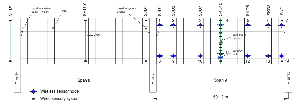
Figure 4. Locations of the wireless SHM system inside the concrete box of the Newmarket Viaduct.
