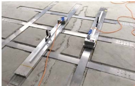
Figure 6. Heating process with infrared heating units (left), strengthened RC slab before grouting (right)
