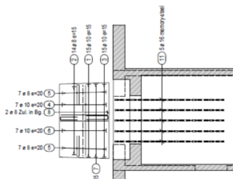
Figure 10. Drawing of horizontal section of strengthened RC slab (left), filling of groove for end-anchorage (right)
