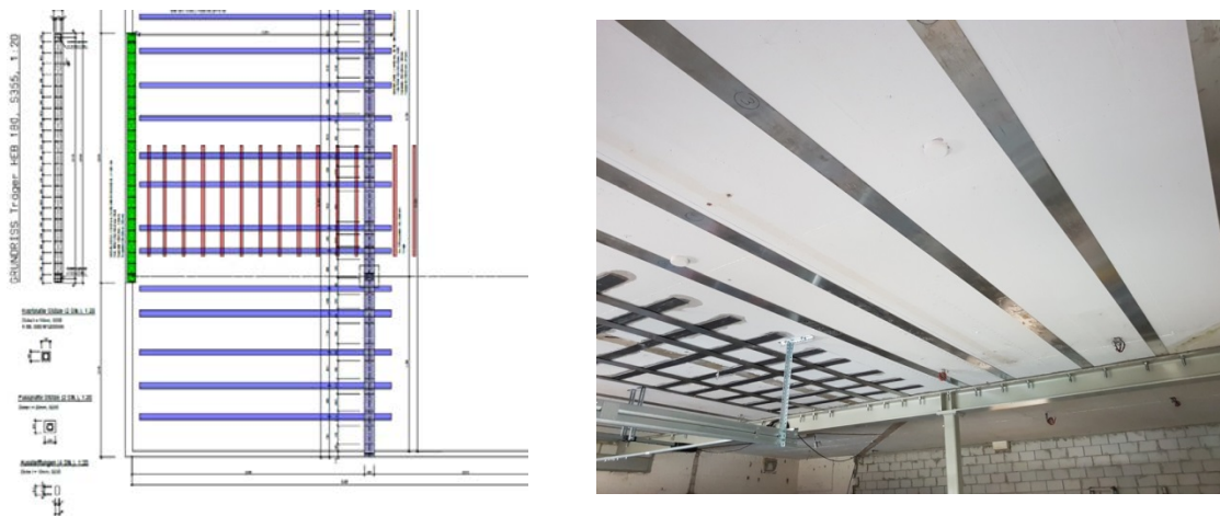
Figure 2. Drawing of horizontal section of strengthened RC slab (left), Finished strengthening project, using re-plate, CFRP strips and a steel beam (right)
